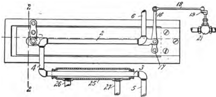
FIG. 192.—The Bullard Thermostat Regulator as arranged for a Stationary Boiler. The U-shaped tube, 2, 3, 4, the lower leg of which passes through the water-feed pipe, 25, is set at the normal water level, as indicated by the broken line above the upper leg. When the boiler level sinks unusually, the pipe elongates on its bed plate as far as the vertical line, 2, 3, thus operating the lever, 16, and closing the by-pass valve, 20, through the link, 18. The construction used on the "Victor" carriage is substantially the same as here shown.
